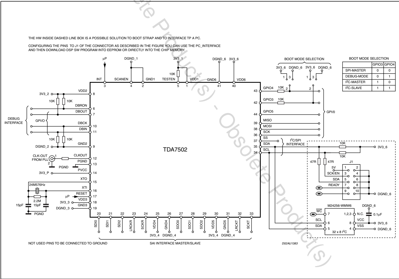
Figure 16. Application schematic for TDA7502
