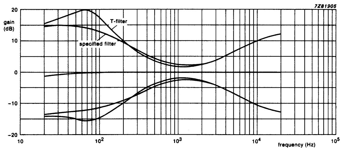
Fig.17 Tone control.
