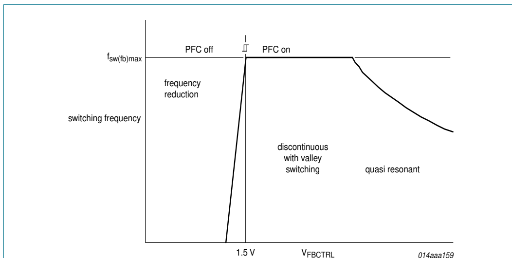
Fig 8. Frequency control of flyback
