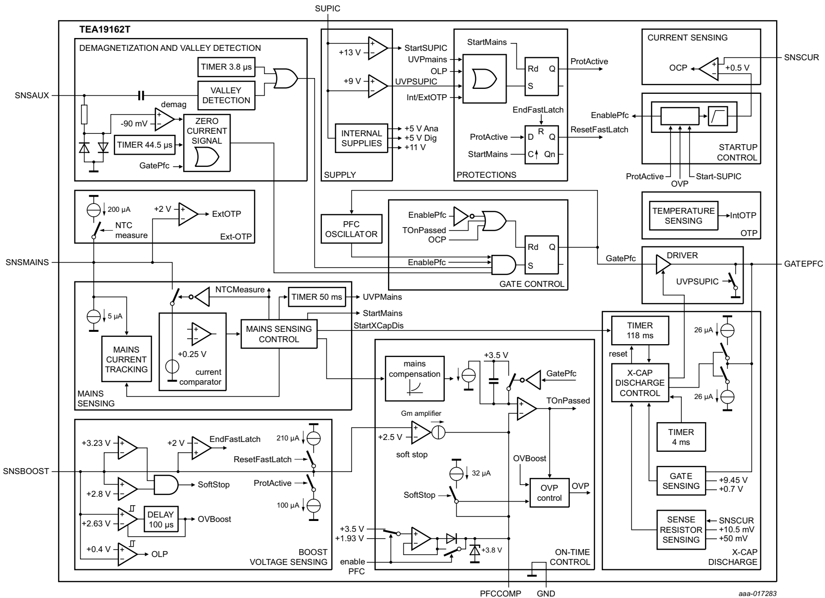
Fig 1. Block diagram
