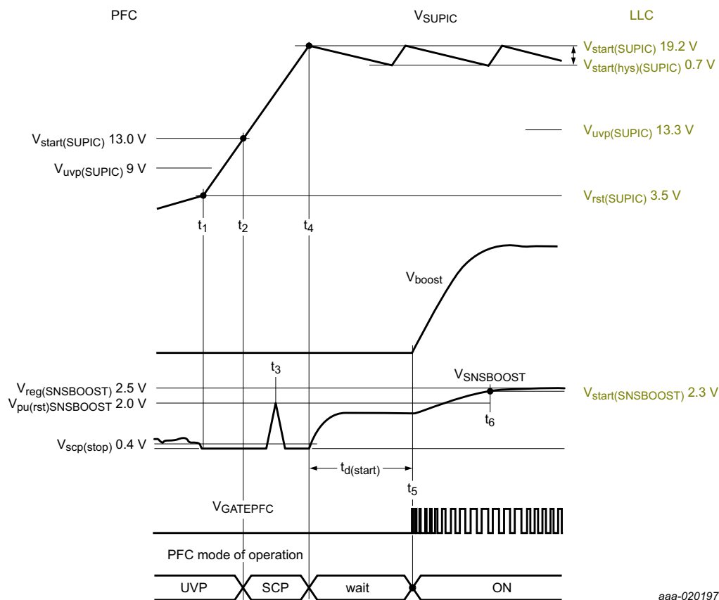
Fig 4. Start-up of the PFC and LLC
