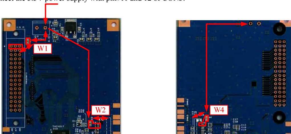
(a)THEVA217-V2 (Top Side)
