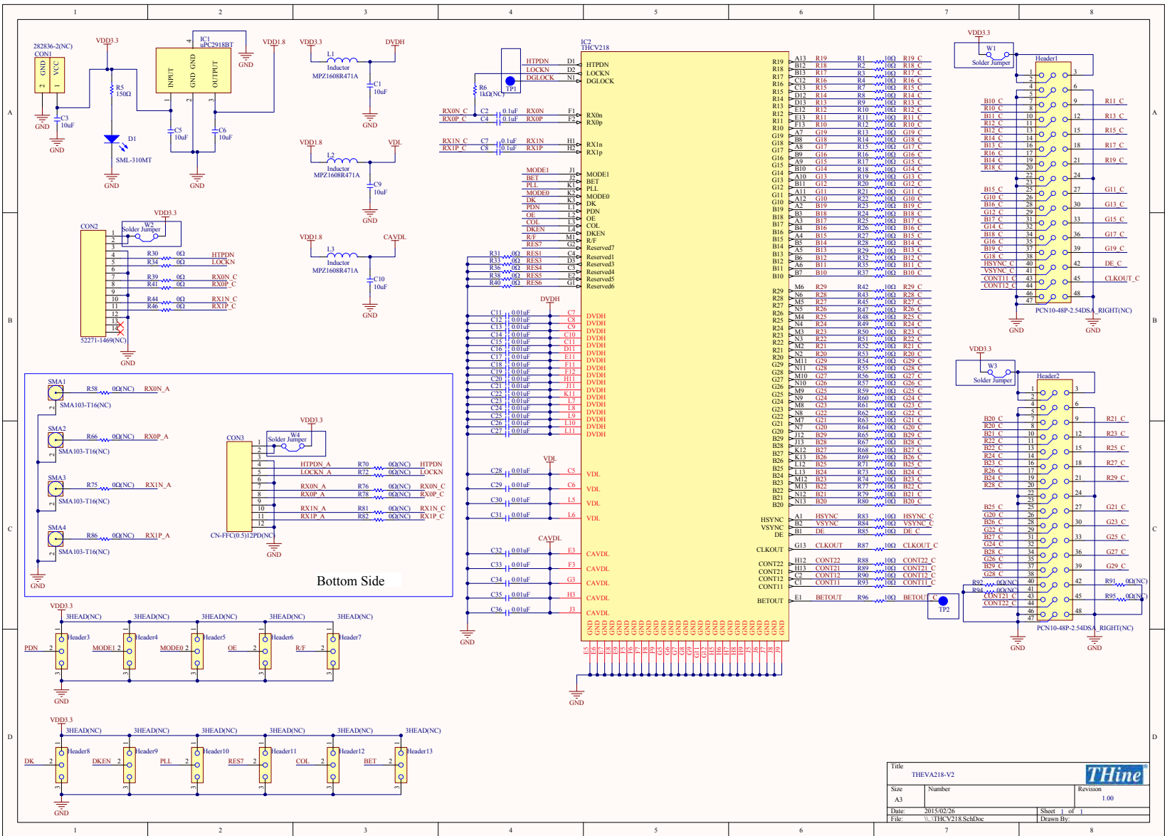
Figure 14 THEVA218-V2 schematic
