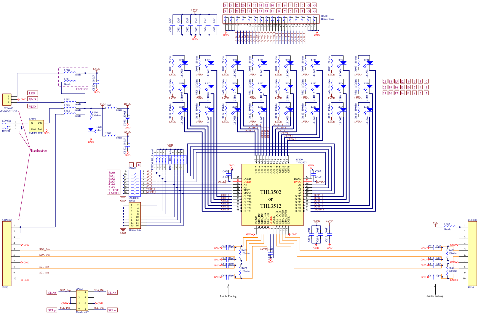
Figure 7 Board schematic
