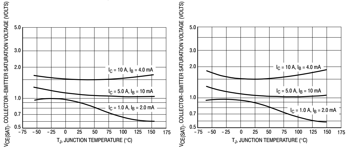
Figure 4. Collector-Emmitter Saturation Voltage
