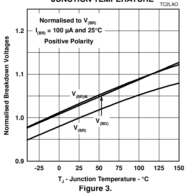
NORMALISED BREAKDOWN VOLTAGES vs JUNCTION TEMPERATURE
