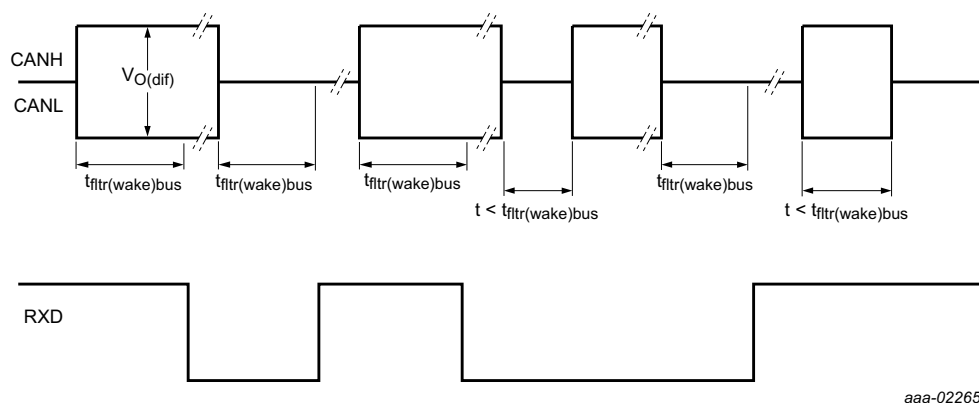
Fig 3. Wake-up timing
