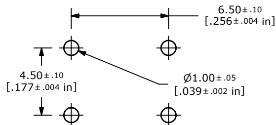
P.C. MOUNTING
