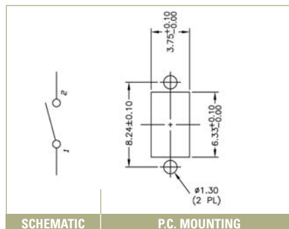
SCHEMATIC
