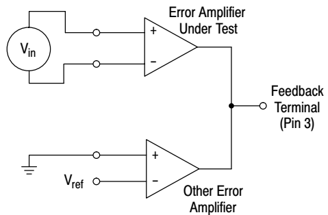
Figure 11. Error-Amplifier Characteristics
