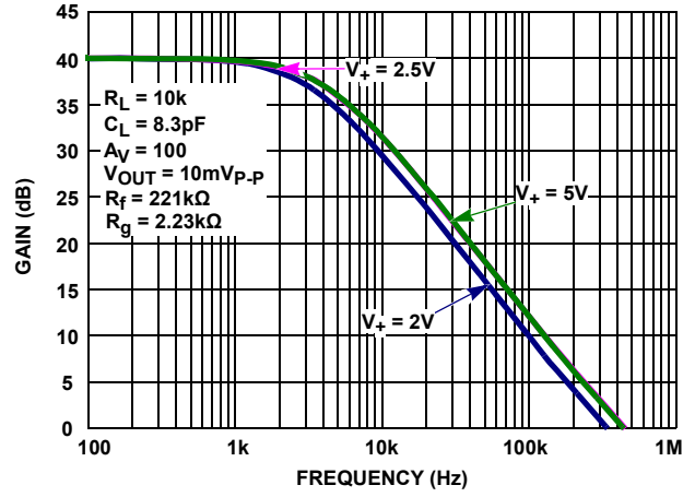
FIGURE 10. GAIN vs FREQUENCY vs SUPPLY VOLTAGE
