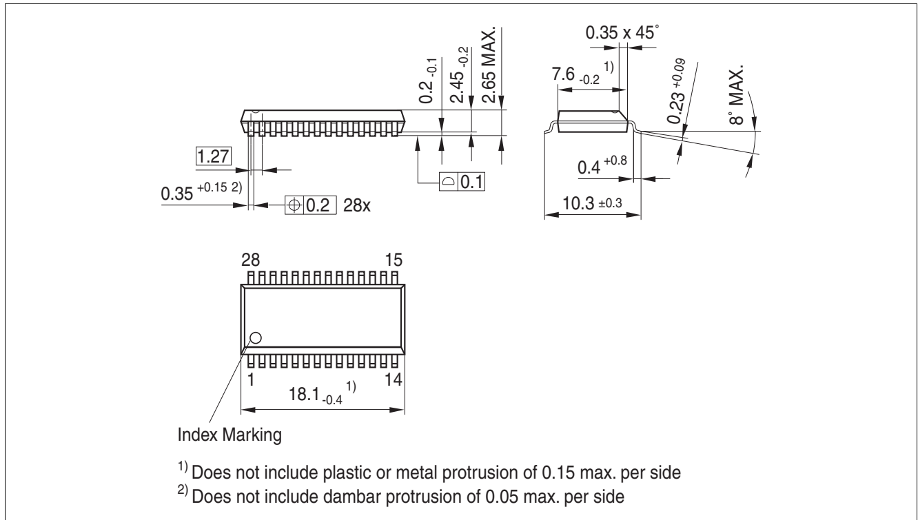
Figure 4 PG-DSO-28
