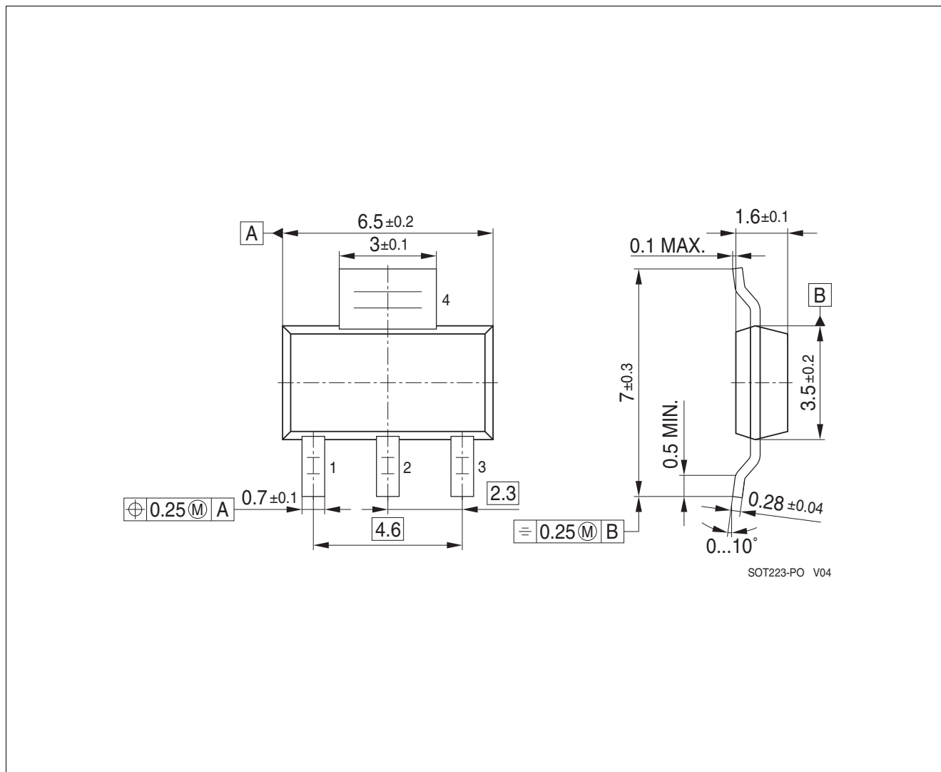
Figure 4 PG-SOT223-4
