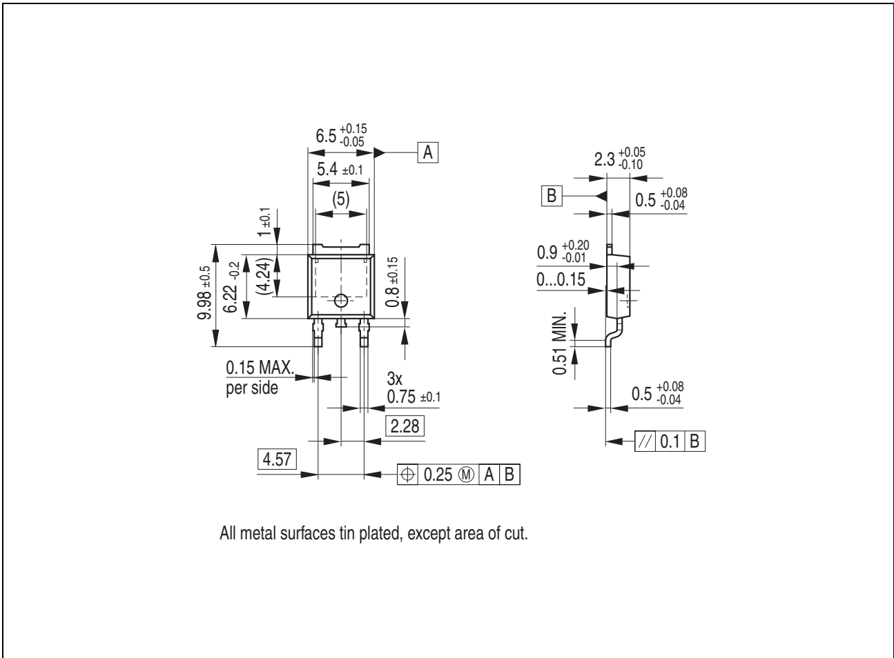
Figure 5 Dimensions PG-T0252-3-11
