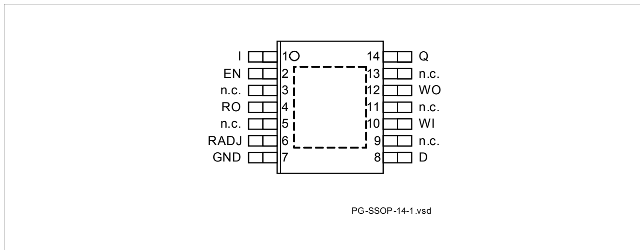
Figure 2 Pin Configuration PG-SSOP-14 EP
