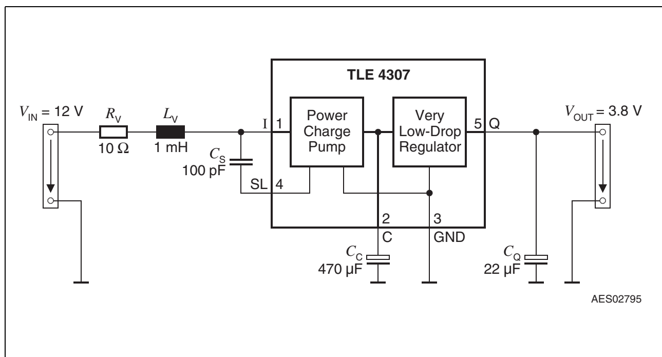
Figure 4 Measurement Circuit
