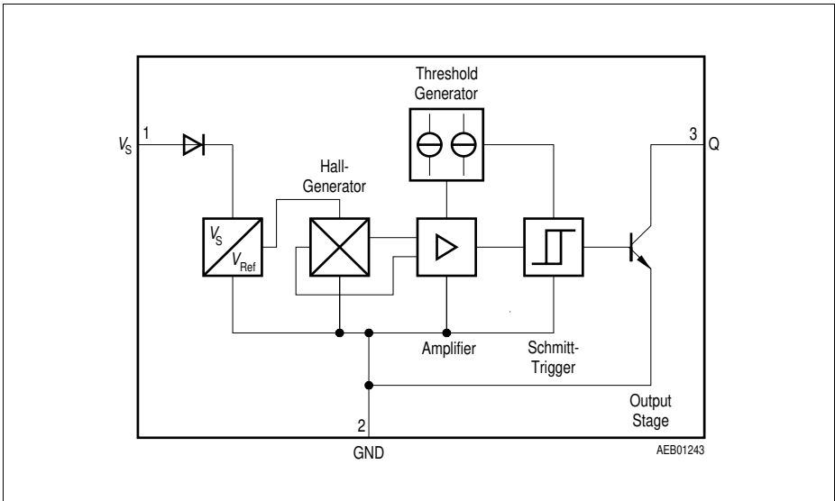
Figure 2 Block Diagram
