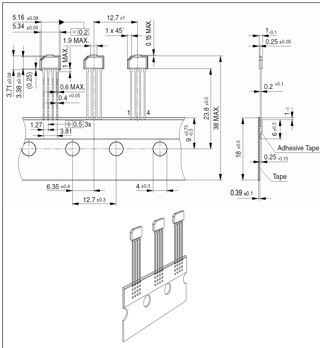
Figure 7 Package Outline
