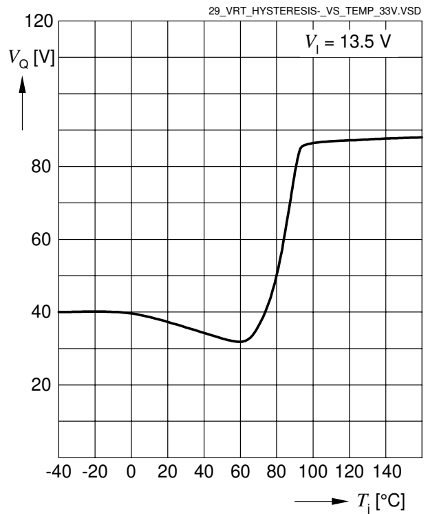
Reset Hysteresis versus Junction Temperature T_J (3.3V-Version)
