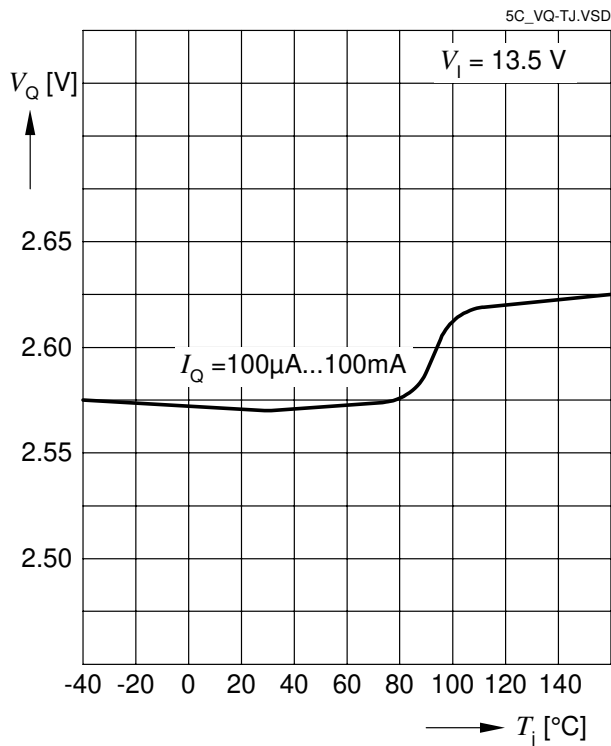
Output Voltage V_Q versus Junction Temperature T_J (2.6V Version)
