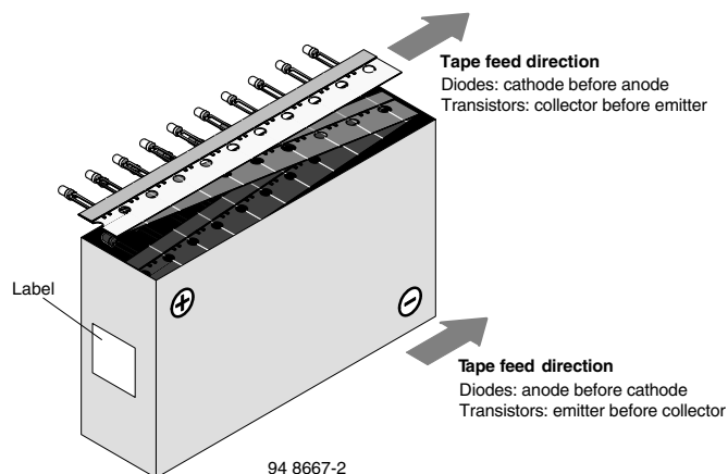
Fig. 9 - Tape Direction
