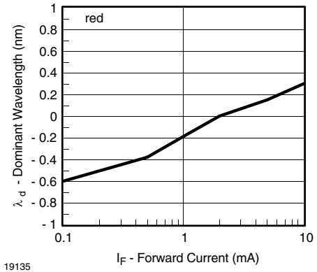
Fig. 15 - Dominant Wavelength vs. Forward Current
