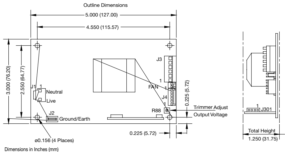
Figure 2: Mechanical Drawing
