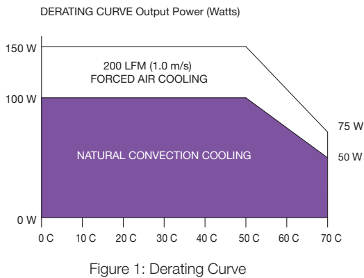
Figure 1: Derating Curve
