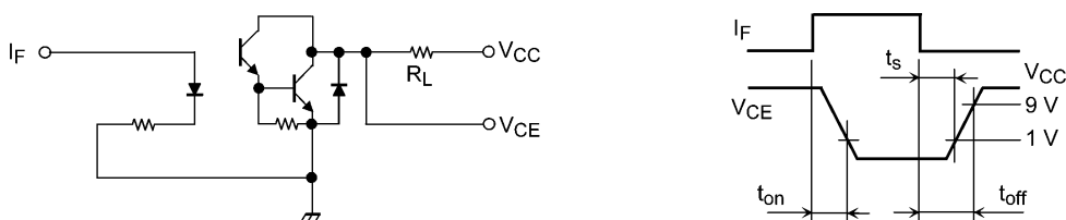
Fig. 10.1 Switching Time Test Circuit and Waveform
