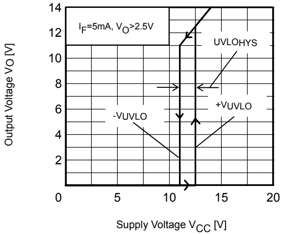
V_O(V_{UVLO})^{**} - V_{CC}
