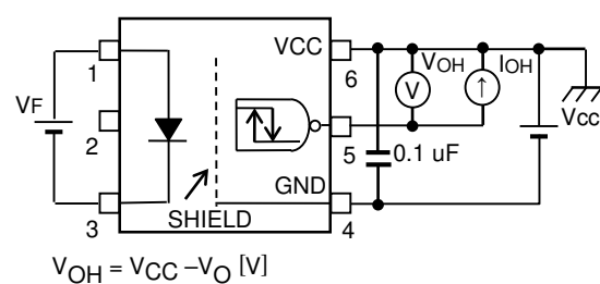
Figure 2: V_{OH} TEST CIRCUIT
