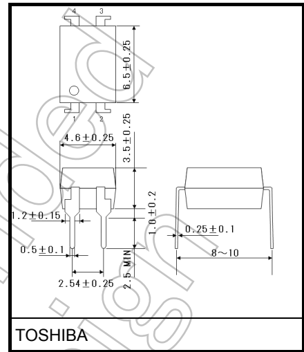
TLP781 Unit: mm
