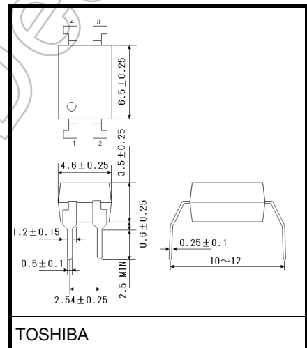
TLP781F Unit: mm
