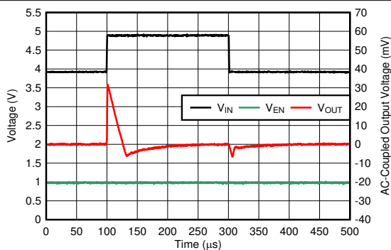
Figure 8-6. VIN Line Transient, I_{OUT} = 1 \text{ mA}
