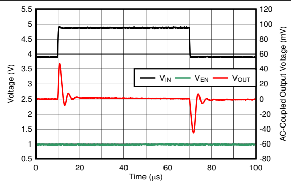
Figure 8-7. VIN Line Transient, I_{OUT} = 30 \text{ mA}
