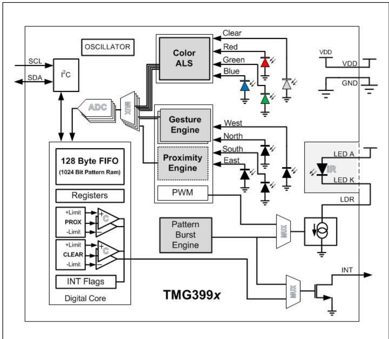
Figure 2: TMG3992 Block Diagram
