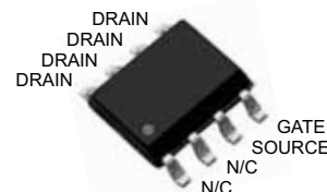
8-Lead SOIC
