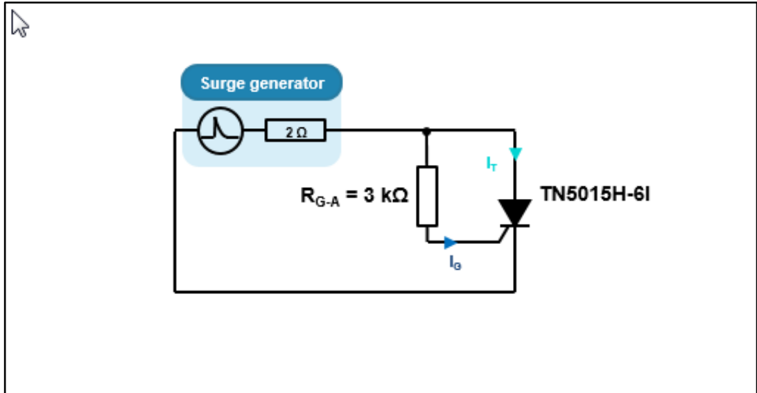
Figure 13: IPP 8/20 \mu s test circuit
