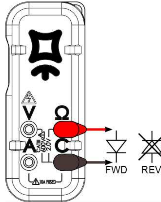
FIGURE 5 DIODE MEASUREMENT
