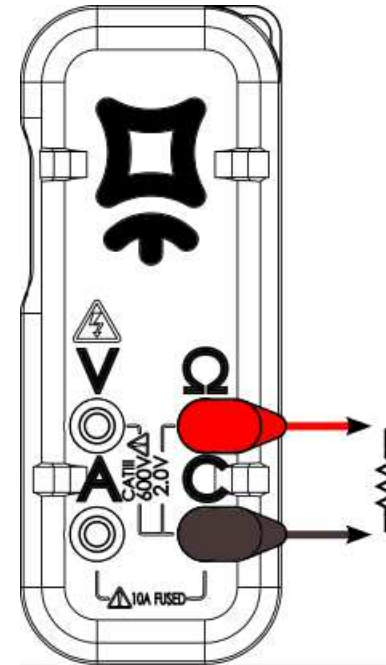
FIGURE 4 RESISTANCE MEASUREMENT
