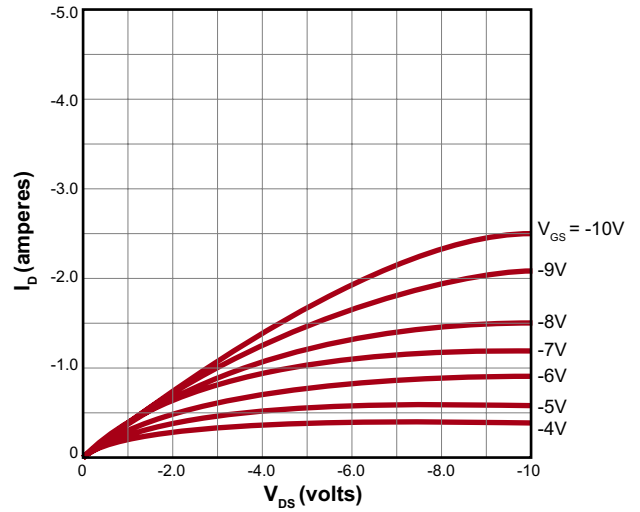
Saturation Characteristics
