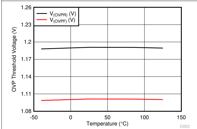
Figure 7-3. OVP Threshold Voltage vs Temperature
