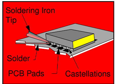
Figure 14: Soldering Technique
