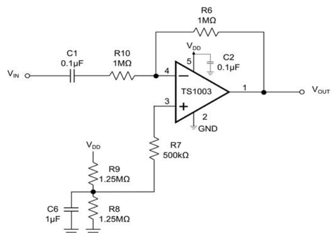
Figure 4. Inverting Configuration
