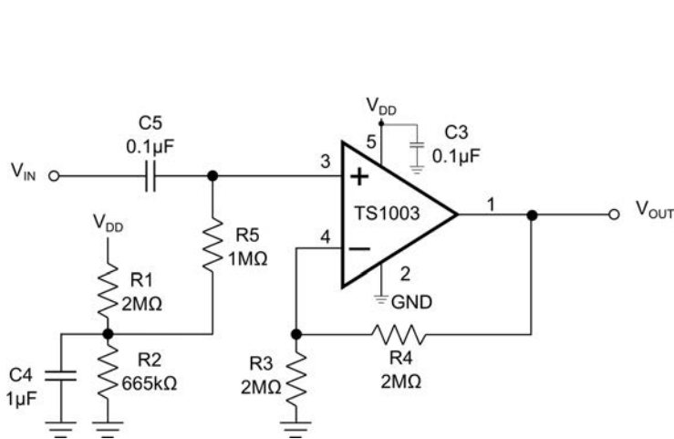
Figure 3. Non-Inverting Configuration
