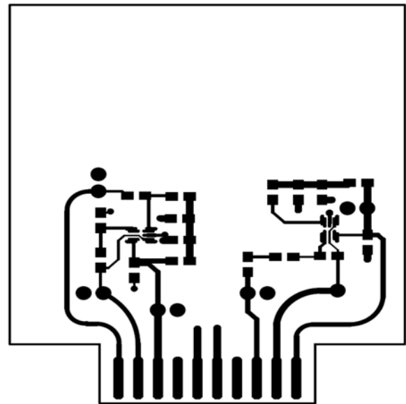
Figure 6. TS1003 Demo Board Top Layer #2
