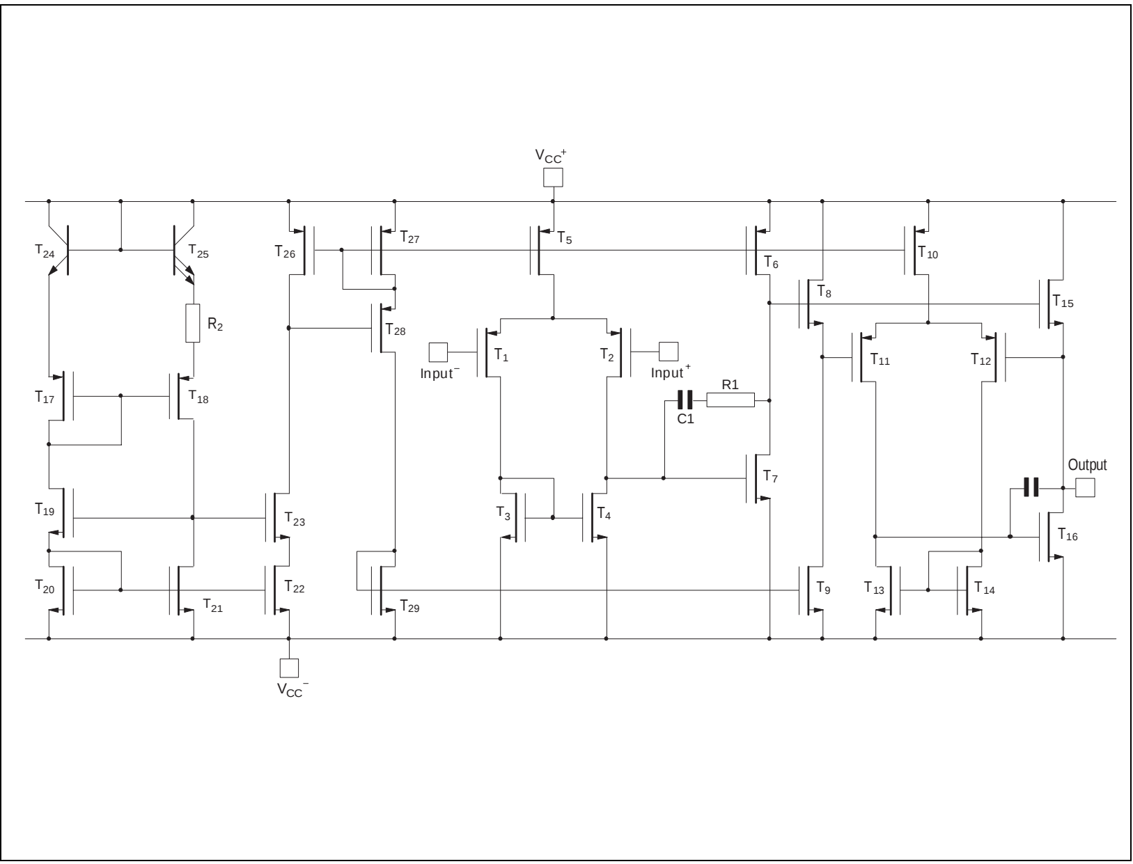
SCHEMATIC DIAGRAM (for 1/2 TS272)
