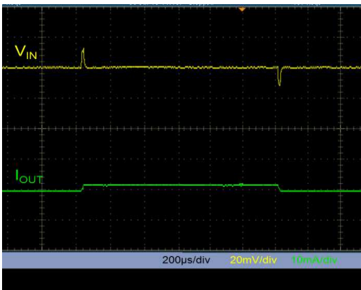
Figure 14: Load transient ( I_{OUT} = \pm 1\text{ mA} )
