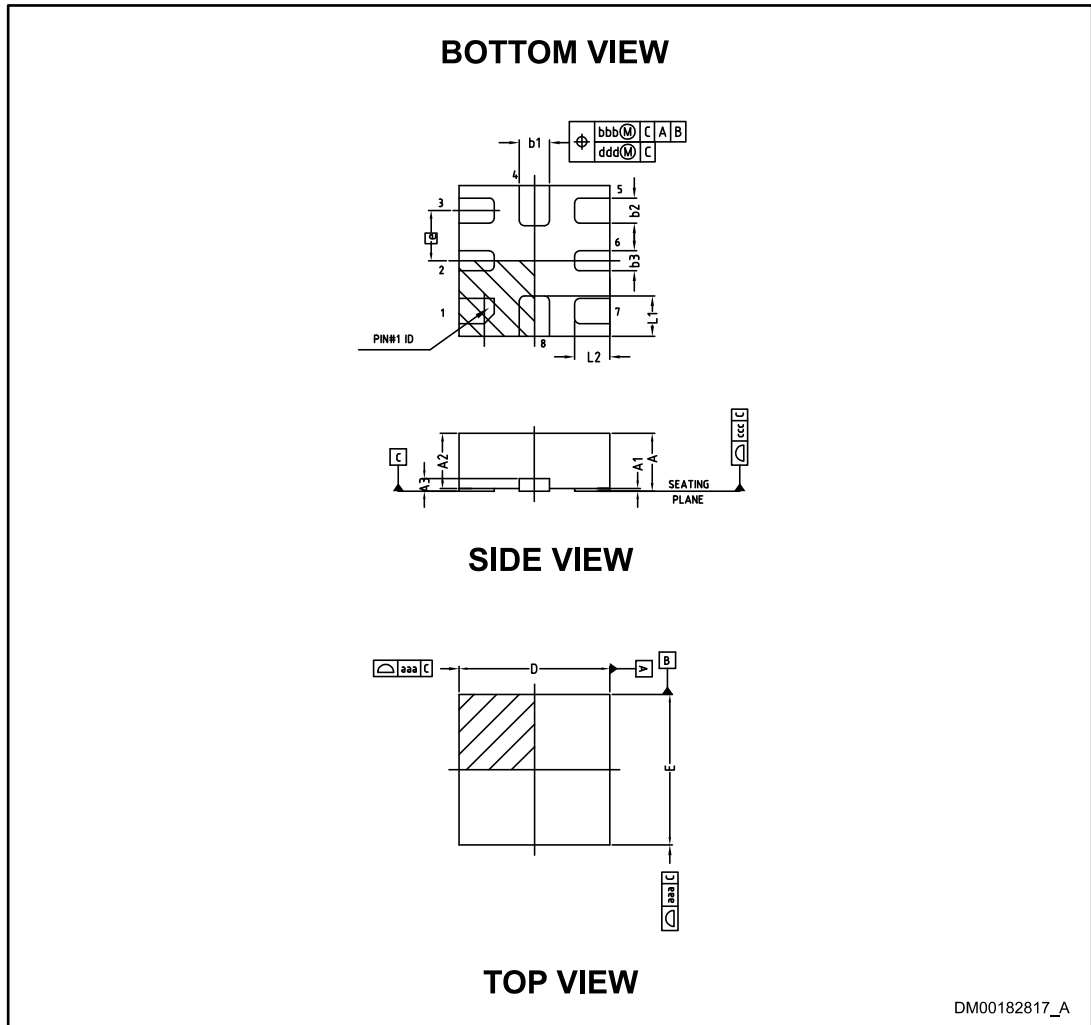
Figure 18: QFN8 package outline
