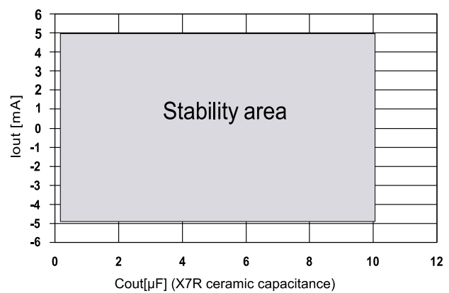
Figure 17: Stability plan
