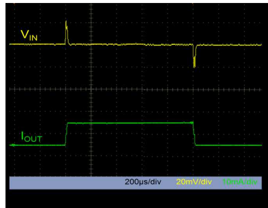
Figure 15: Load transient ( I_{OUT} = \pm 5\text{ mA} )
