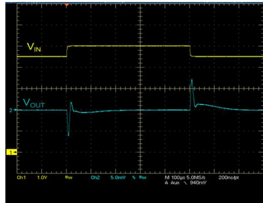
Figure 13: Line transient ( I_{OUT} = 1\text{ mA} )
