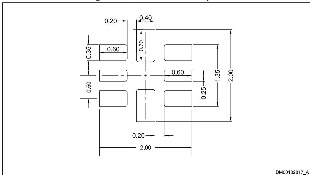
Figure 19: QFN8 recommended footprint
