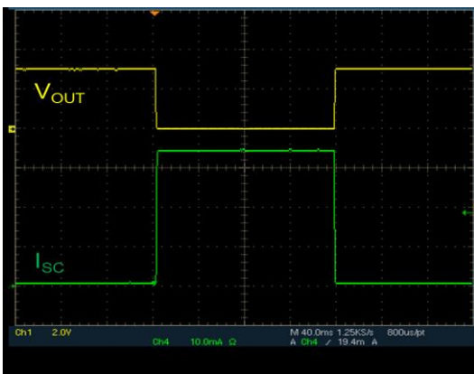
Figure 16: Short-circuit response
