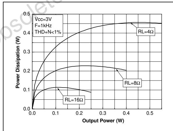
Figure 54: Power dissipation vs. output power. headphone output one channel
