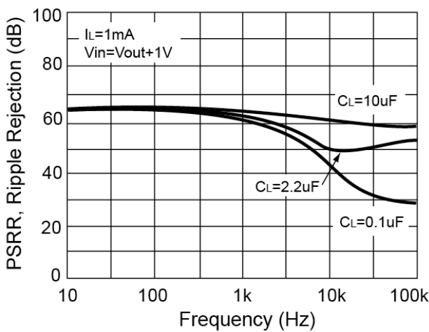
Figure 5. Ripple Rejection vs. Frequency
