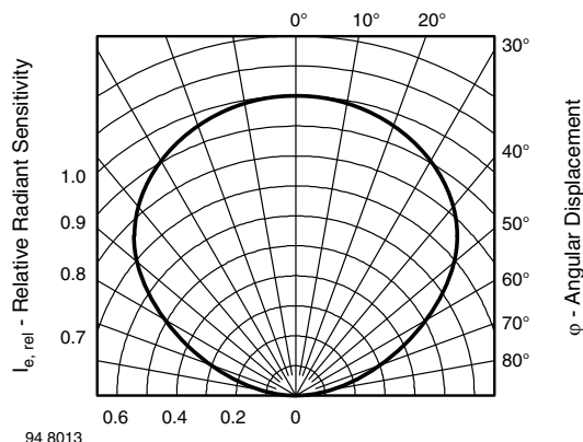
Fig. 2 - Radiant Characteristics I_{rel} = f(\varphi)
