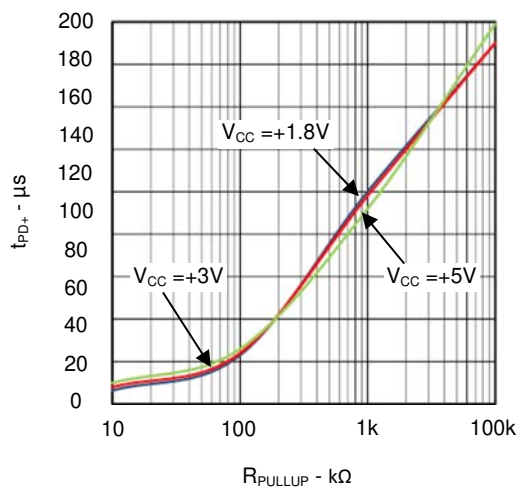
TS9001-2 Propagation Delay (t PD+ ) vs Pullup Resistance
