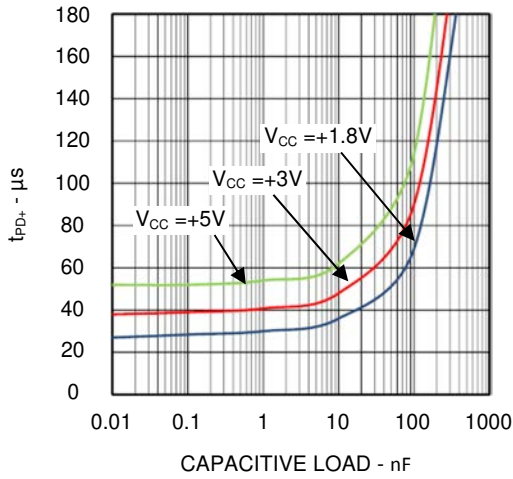
TS9001-1 Propagation Delay (t PD+ ) vs Capacitive Load
