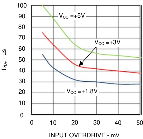
TS9001-1 Propagation Delay (t PD+ ) vs Input Overdrive
