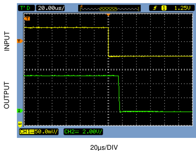
Propagation Delay (t PD- ) at V CC = +5V
