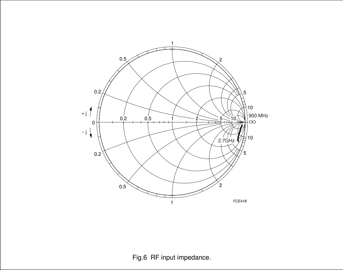
RF input impedance
