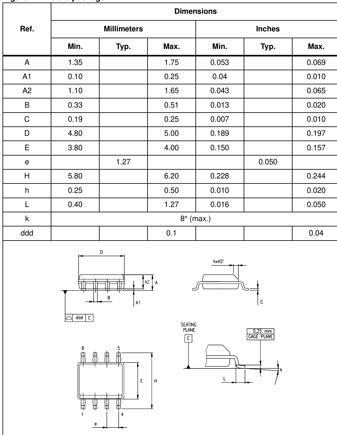
Figure 24. SO-8 package
