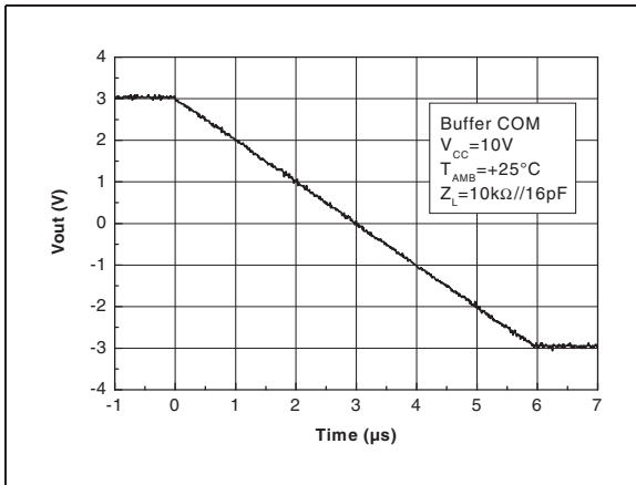
Figure 32. Large signal response - buffer COM
