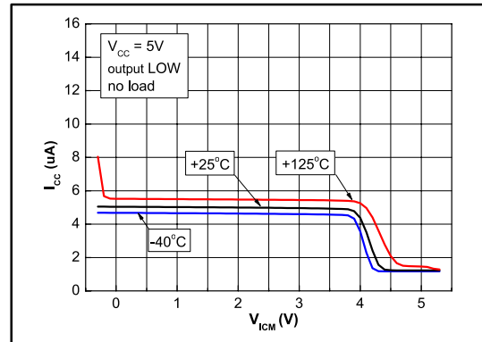
Figure 6: Current consumption vs. common-mode voltage, output low
