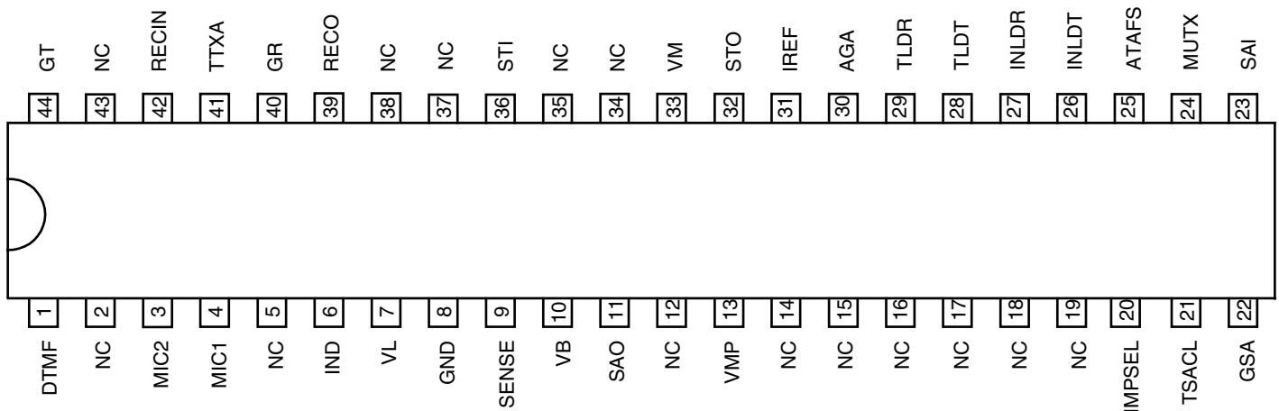
Figure 2-1. Pinning SSO44
