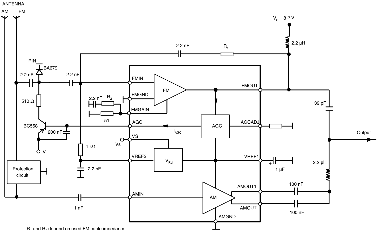
Figure 17. Application Circuit
