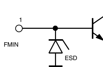
Figure 4. Internal Circuit at Pin FMIN
