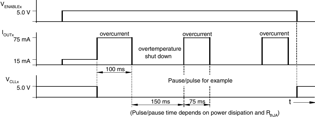
Figure 7-2. Overcurrent Protection
